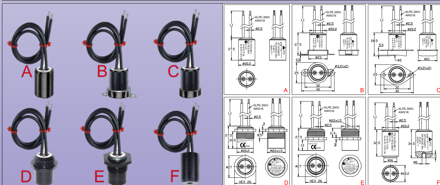
4VB main types with wires
